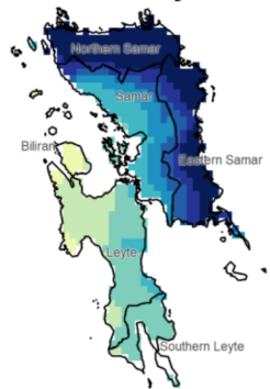
RX5day
