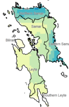
RX1day
